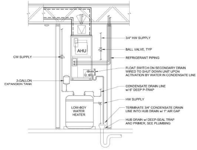
1 HVAC-MECHANICAL CLOSET DETAIL 2 P301 SCALE: 1/4" = 1'-0"
