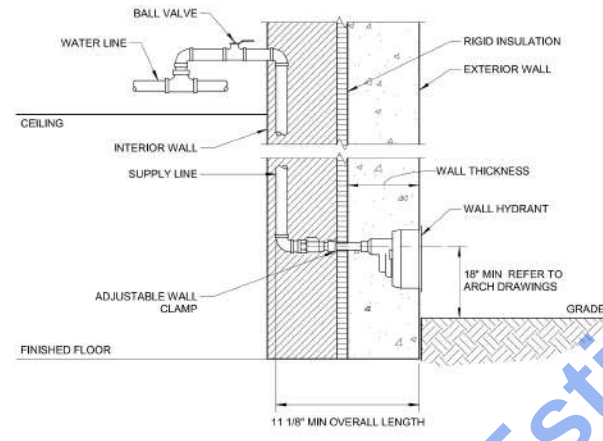
4 WALL HYDRANT PIPING DETAIL P301 SCALE: NTS
