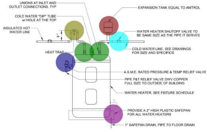
5 WATER HEATER PIPING DETAIL P301 SCALE: NTS
