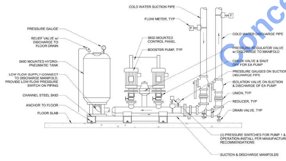
2 DOMESTIC WATER PRESSURE BOOSTER DETAIL P301 SCALE: NTS
